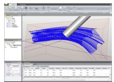
3D-Simulation in StairCon CAM 5+
